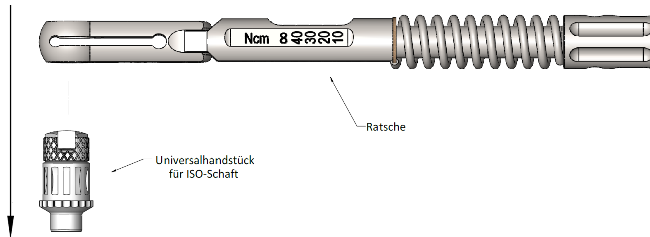
UNIVERSALHANDINSTRUMENT – RATSCHKE
